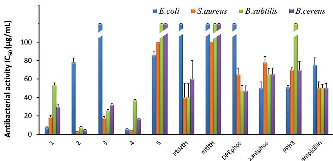
Fig. 3 In vitro antibacterial activity of 1–5, and their ligands atdztH, mtftH, DPEphos, xantphos, and PPh _3 in free form, expressed as half-minimum inhibitory concentration (IC _{50} ) values ( \mu\text{g mL}^{-1} ) provided by a nonlinear curve fit-growth/sigmoidal-dose response on the experimental optical density data. Values are expressed as mean \pm standard deviation (SD) of three replicate measurements (with the exception of values higher than 100 \mu\text{g mL}^{-1} ).
