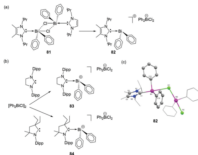
Fig. 27 Syntheses of carbene-stabilized bismuth cations 82–84 (a) and (b); (c) solid-state structure of 82 .
