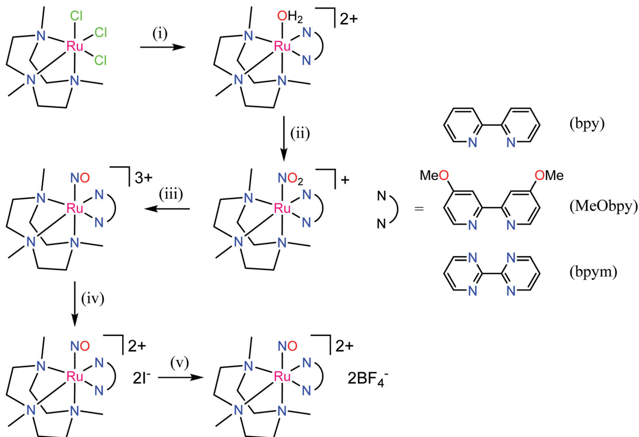
Scheme 3 Synthetic route to \{Ru(NO)\}^7 complexes. Reagents and conditions: (i) bpy, MeObpy or bpym, Zn powder, aqueous solution; (ii) NO_2^- ; (iii) HOTf; (iv) acetone, I^- ; (v) Dowex 22 ( BF_4^- ), then lyophilization.
