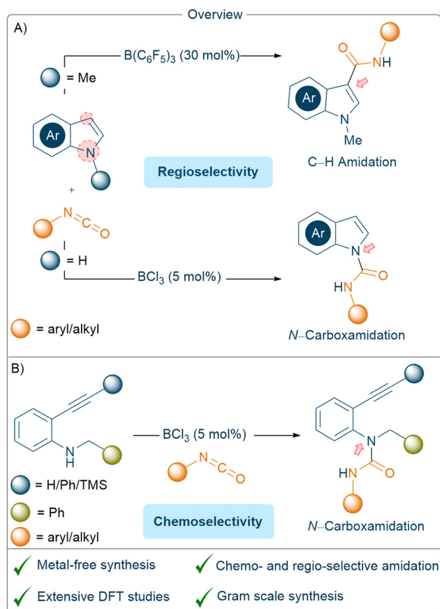
Scheme 2 An overview of indole amidation reactions: (A); an intramolecular reaction vs. N-H insertion of 2-alkynyl anilines, with isocyanates (B).
