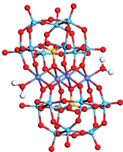
Fig. 133 Structural model of [\text{Ni}_4(\text{H}_2\text{O})_2(\text{SiW}_9\text{O}_{34})_2]^{12-} ( M = \text{Ni} ; \text{W} : blue, \text{O} : red; \text{S} : yellow; \text{H} : white; \text{M} : dark blue). Reprinted with permission from ref. 1600. Copyright 2012 RSC.
