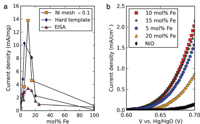
Fig. 37 (a) Electrochemical oxygen evolution activity at a fixed overpotential of 360 mV for the varying synthesis methods and compositions of mixed metal oxide electrocatalysts. (b) Geometric area-normalised polarisation (scan rate = 1\text{ mV s}^{-1} ) data of mixed Ni–Fe oxide catalysts (synthesised by the EISA method) showing the highest activity for 10 mol % Fe oxide. Reproduced with permission from ref. 736 Copyright American Chemical Society 2012.
