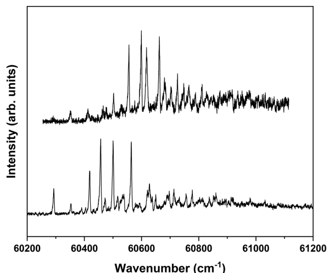
Fig. 6 ZEKE-PFI spectrum obtained for excitation at the tentatively assigned S_1 \leftarrow S_0 origin transition (31 281.3 \text{cm}^{-1} ) of MS (bottom) and at 31 353.9 \text{cm}^{-1} (top) where an unassigned S_1 vibrational level of the anti/trans conformer is excited.
