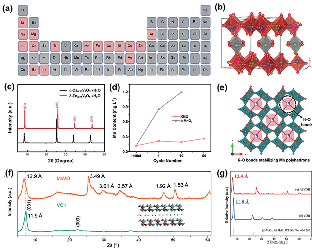
Fig. 1 (a) Periodic table of cations (marked with pink color) that have been introduced into cathode materials. (b) Crystal structure of Zn 0.25 V 2 O 5 ·nH 2 O. Reproduced with permission. 38 Copyright 2016, Springer Nature. (c) XRD pattern of Ca 0.25 V 2 O 5 ·nH 2 O. Reproduced with permission. 36 Copyright 2018, Wiley-VCH. (d) Element content of dissolved Mn 2+ in a 2 M ZnSO 4 aqueous electrolyte during the cycling of KMO and α-MnO 2 . (e) Schematic of the incorporation of K + ions stabilizing the Mn polyhedrons. (d and e) Reproduced with permission. 68 Copyright 2019, Wiley-VCH. (f) XRD patterns of MnVO and VOH. Reproduced with permission. 69 Copyright 2019, Royal Society of Chemistry. (g) XRD patterns of Al-VOH and VOH. Reproduced with permission. 40 Copyright 2020, Elsevier.
