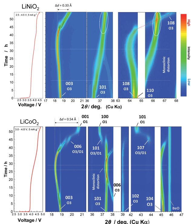
Fig. 2 Contour plots for selected ranges obtained from the in situ XRD patterns of \text{LiNiO}_2 and \text{LiCoO}_2 at a rate of 5 mA \text{g}^{-1} , and corresponding initial charge curves in electrochemical cells are also shown. The original in situ XRD data are shown in ESI Fig. S3.†
