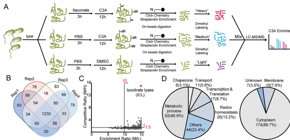
Fig. 2 Quantitative chemoproteomic profiling of itaconated proteins by C3A in S. enterica lysates. (A) Workflow for the triplex dimethylation-based quantitative chemoproteomic profiling of itaconated proteins in S. enterica by C3A. (B) Overlap of the itaconated proteins identified by C3A in four biological replicates. (C) Distribution of the averaged enrichment and competition ratios of the C3A-labeled proteins. (D) Bioinformatics analysis of the prominent 197 itaconated protein targets in terms of functional annotation and cellular location.
