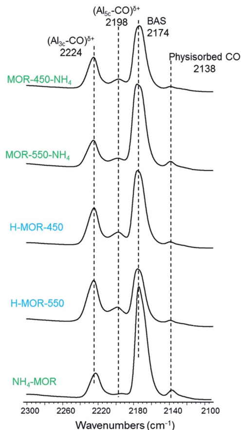
Fig. 5 FTIR spectra of adsorbed carbon monoxide over activated parent ammonium form \text{NH}_4\text{-MOR} , H-MOR-450, H-MOR-550, MOR-450- \text{NH}_4 and MOR-550- \text{NH}_4 . The names of the samples refer to the form of the zeolite prior to heat treatment in the IR setup.
