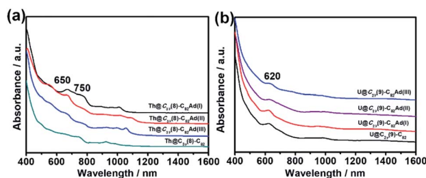
Fig. 3 UV-vis-NIR absorption spectra of (a) Th@C_{3v}(8)-C_{82} and Th@C_{3v}(8)-C_{82}Ad(I, II, III) and (b) U@C_{2v}(9)-C_{82} and U@C_{2v}(9)-C_{82}Ad(I, II, III) in CS_2 .
