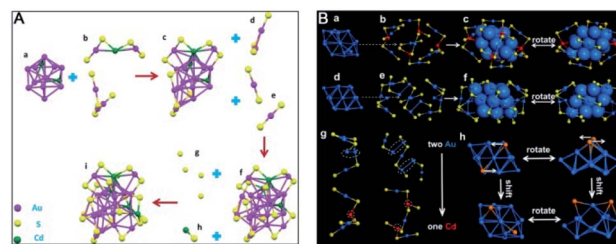
Fig. 14 Anatomy of the structure of (A) \text{Au}_{20}\text{Cd}_4(\text{SH})(\text{SR})_{19} and (B) \text{Au}_{26}\text{Cd}_4(\text{CHT})_{22} nanoclusters (reproduced from ref. 92 with permission from John Wiley and Sons, Copyright (2018) and ref. 93 with permission from the American Chemical Society, Copyright (2019)).
