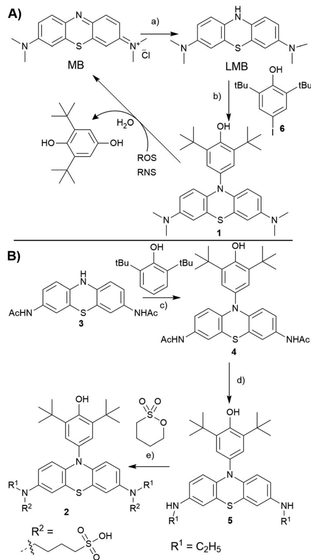
Scheme 1 (A) Synthesis of hydrophobic BHP-LMB ( 1 ), (B) bis-sulfonated hydrophilic BHP-LMB ( 2 ). (a) K 2 CO 3 , Na 2 S 2 O 4 in DCM/H 2 O at 40 °C under N 2 , (60%) (b) Pd 2 (dba) 3 , DPPF, 6 , NaO t Bu in toluene at 110 °C under N 2 , (10%, air sensitive) (c) NaIO 4 in DCM/AcOH, BHP, at 40 °C (34%); (d) BH 3 ·SMe 2 in toluene at 110 °C (87%); (e) 1,4-butanefulfonate, DIPEA in MeCN at 80 °C under N 2 (15%).
