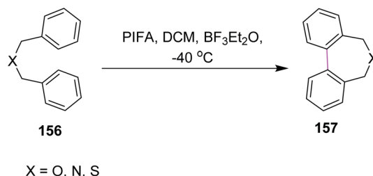
Scheme 65 Oxidative coupling of benzyl ethers with PIFA.
