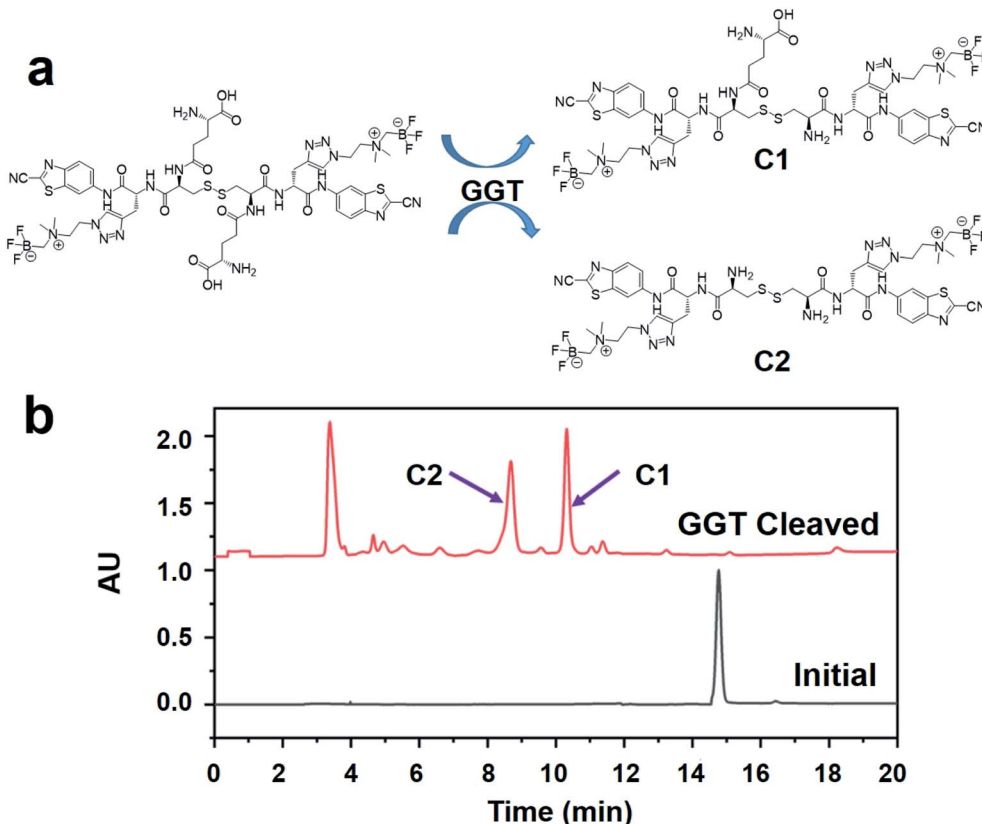
Fig. 2 (a) Schematic illustration of GGT-controlled cleavage of (GCPA) 2 to form two enzymatic products. (b) HPLC analysis of 250 μM (GCPA) 2 incubated with 0 (black) or 100 U L -1 of GGT (red) at 37 °C for 30 min.
