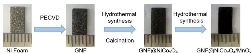
Fig. 1 Schematic of the synthesis process of \text{GNF@NiCo}_2\text{O}_4/\text{MnO}_2 .
