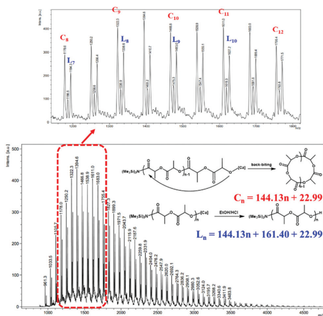
Fig. 4 MALDI-TOF mass spectrum (major population: Na + ) of the PLA sample ( M_{n, GPC} = 2900 \text{ g mol}^{-1} , M_w/M_n = 1.88 ) prepared with catalyst 1 ( C(\text{cyclic}) = 144.13n + 22.99 , L(\text{linear}) = 144.13n + 161.40 + 22.99 , where n is the degree of polymerization, M_{LA} = 144.13 \text{ g mol}^{-1} , M_{NH(SiMe_3)_2} = 161.40 \text{ g mol}^{-1} , M_{Na} = 22.99 \text{ g mol}^{-1} ).
