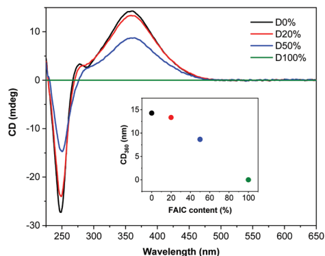
Fig. 3 CD (THF, 0.5 mg mL -1 ) spectra of P(PAIC) 20 - b -(P(MAIC) y - co -P(FAIC) z ) 30 with 0, 20, 50 and 100 mol% of FAIC.
