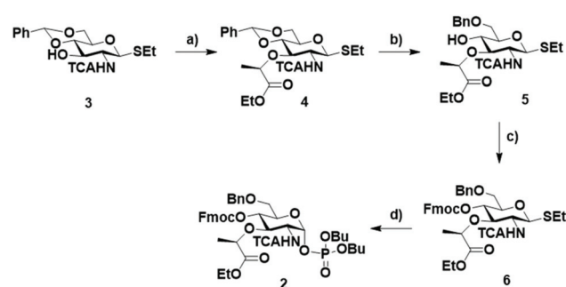
Scheme 2 Synthesis of the MurNac BB 2 . Reagents and conditions: (a) (–)-ethyl ( S )-2-trifluoromethylsulfonyloxy propionate, NaH, DMF/ \text{CH}_2\text{Cl}_2 , 0^\circ\text{C} \rightarrow \text{rt} , 53%; (b) \text{Me}_3\text{N}\cdot\text{BH}_3 , \text{BF}_3\cdot\text{OEt}_2 , \text{CH}_3\text{CN} , 0^\circ\text{C} \rightarrow \text{rt} , 65%; (c) FmocCl, pyridine, \text{CH}_2\text{Cl}_2 , rt, 93%; (d) (\text{BuO})_2\text{P}(\text{O})\text{OH} , NIS, TFOH, 0^\circ\text{C} \rightarrow \text{rt} , 83%.
