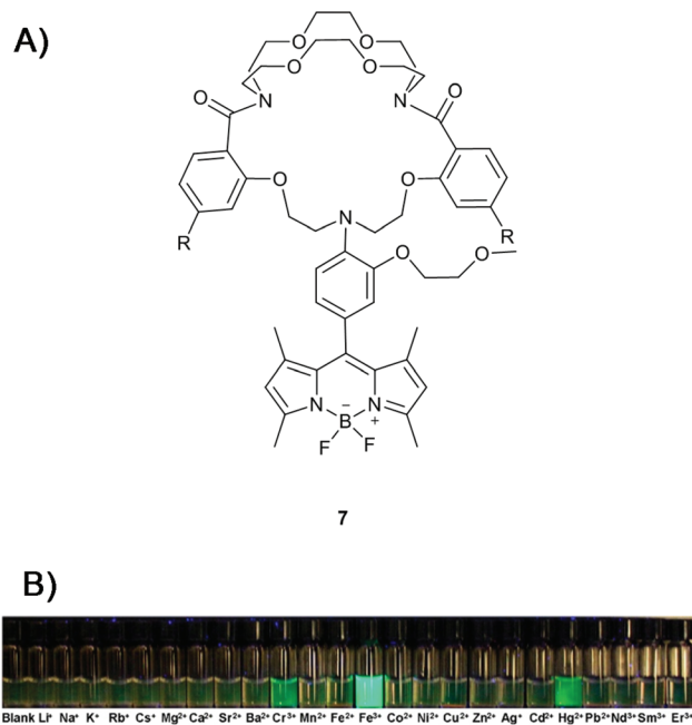
Fig. 4 (A) Cryptand-bodipy based sensor 7 for the detection of \text{Fe}^{3+} . (B) Naked-eye fluorescence responses of 7 ( 7 \mu\text{M} ) in \text{H}_2\text{O}-\text{CH}_3\text{CN} (9 : 1) upon addition of 100 equiv. of various metal cations ( \lambda_{\text{ex}} = 365 \text{ nm} ). Reproduced with permission from ref. 29, copyright American Chemical Society.
