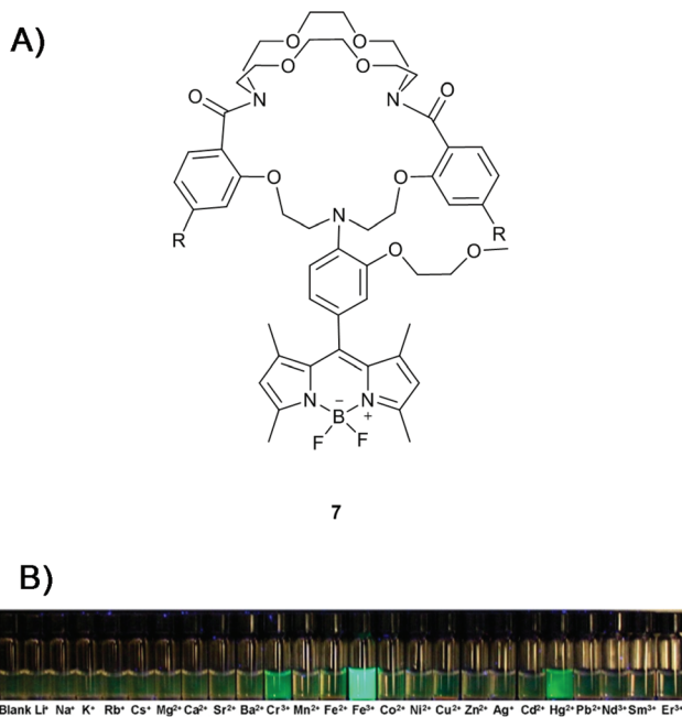
Fig. 4 (A) Cryptand-bodipy based sensor 7 for the detection of Fe 3+ . (B) Naked-eye fluorescence responses of 7 (7 μM) in H 2 O-CH 3 CN (9:1) upon addition of 100 equiv. of various metal cations ( \lambda_{\text{ex}} = 365 \text{ nm} ). Reproduced with permission from ref. 29, copyright American Chemical Society.
