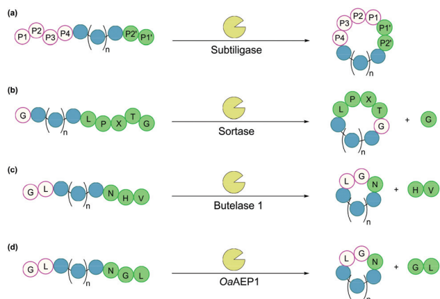
Fig. 6 Enzymatic methods for backbone cyclisation (in some cases great recognition sequences may vary): (a) subtiligase, (b) sortase, (c) butelase 1, and (d) OaAEP1.
