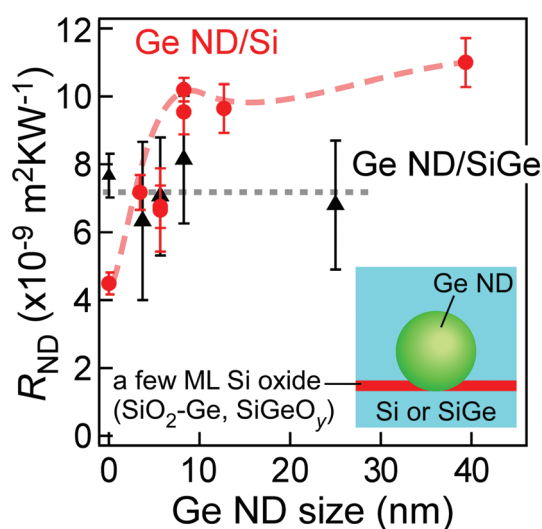
Fig. 4 The Ge ND size dependence of R_{\text{ND}} of the Ge ND/Si films (the red circles) and the Ge ND/ \text{Si}_{0.75}\text{Ge}_{0.25} films (the black triangles). The dashed and dotted curves are the eye-guides.
