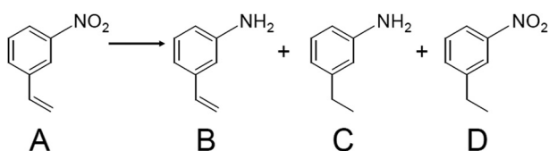
Scheme 10 Hydrogenation of 3-nitrostyrene using metal catalysts. The reaction was conducted under \text{H}_2 atmosphere in toluene. A = 3-nitrostyrene, B = 3-vinylaniline, C = 3-ethylaniline, D = 3-ethylnitrobenzene.
