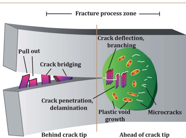
Fig. 11 Toughening mechanisms in epoxy composites reinforced with 2D nanomaterials.
