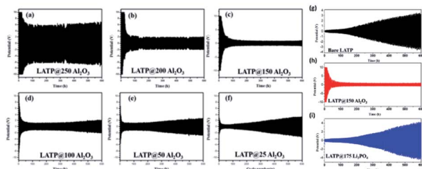
Fig. 18 Electrochemical behavior of \text{Al}_2\text{O}_3 ALD coated LTP/Li symmetrical cells after (a) 250, (b) 200, (c) 150, (d) 100, (e) 50, and (f) 25 cycles at a current density of 0.01 \text{ mA cm}^{-2} , where each cycle takes 2 h for lithium stripping and plating, (g) cycling behavior and voltage profile of bare LTP/Li in the 1st, 100th, 200th, and 300th cycles, (h) cycling behavior and voltage profile of LTP@150 \text{Al}_2\text{O}_3 /Li in the 1st, 100th, 200th, and 300th cycles, and (i) cycling behavior and voltage profile of LTP@175 \text{Li}_3\text{PO}_4 /Li in the 1st, 100th, 200th, and 300th cycles. 51
