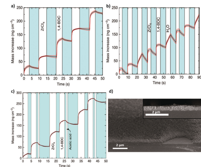
Fig. 8 Mass gain as a function of time measured in situ in the ALD/MLD process with a quartz crystal microbalance (QCM). The red lines show the standard deviations for the QCM data ( n = 16 ), and in blue the N 2 purge step. (a) Alternation between ZrCl 4 and 1,4-BDC pulses separated by N 2 purges. (b) Alternation between ZrCl 4 , 1,4-BDC and water. (c) ALD/MLD process in which a modulation step with acetic acid is included. (d) Cross-section SEM images of the same surface viewed at 45° and 90° angles. Reproduced from ref. 60 with permission from The Royal Society of Chemistry.
