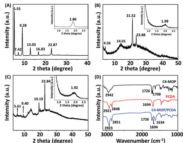
Fig. 4 XRD spectra of (A) PCDA, (B) C4-MOP, and (C) C4-MOP/PCDA assemblies. Insets in (A), (B), and (C) correspond to the results in the small angle region. (D) FT-IR spectra of PCDA, C4-MOP, and C4-MOP/PCDA assemblies.
