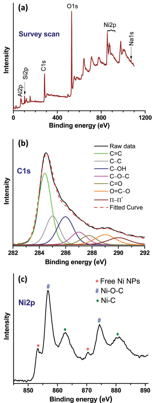
Fig. 4 XPS studies of freshly prepared Ni-rGO-zeolite catalyst. (a) Survey scan, (b) high resolution C1s, and (c) high resolution Ni2p spectra.
