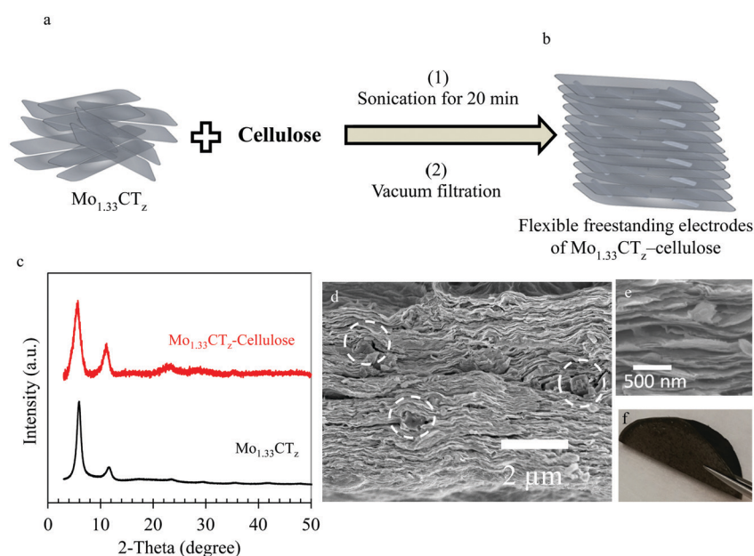
Fig. 1 Synthesis, structure, and morphology of \text{Mo}_{1.33}\text{CT}_z –cellulose composite film (L- \text{Mo}_x\text{C} -45% Cel): (a) and (b) show a schematic illustration of the synthesis method for the \text{Mo}_{1.33}\text{CT}_z –cellulose freestanding electrodes. (c) XRD patterns of the pristine (black) and \text{Mo}_{1.33}\text{CT}_z –cellulose composite (red). (d) and (e) Cross-section SEM images of a \text{Mo}_{1.33}\text{CT}_z –cellulose composite film at low and high magnification, respectively. The white circles in (d) shows cellulose imbedded between the MXene layers. (f) Photo of the freestanding \text{Mo}_{1.33}\text{CT}_z –cellulose film, showing its flexibility.
