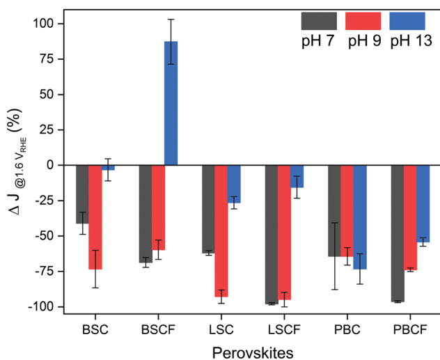
Fig. 3 Results of potential stability tests, where the changes of current density are plotted after 500 cycles of potential steps from 1.0 to 1.6 V_{RHE} holding each potential for 10 seconds. This measurement was carried out in electrolytes of pH 7, 9, and 13.
