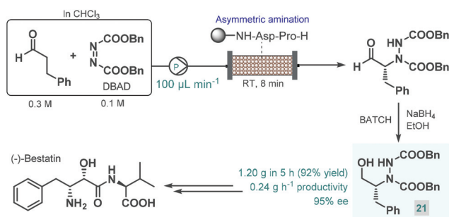
Scheme 9 Continuous flow enantioselective synthesis of a key (-)-bestatin intermediate using a solid supported peptide as chiral organocatalyst. 75
