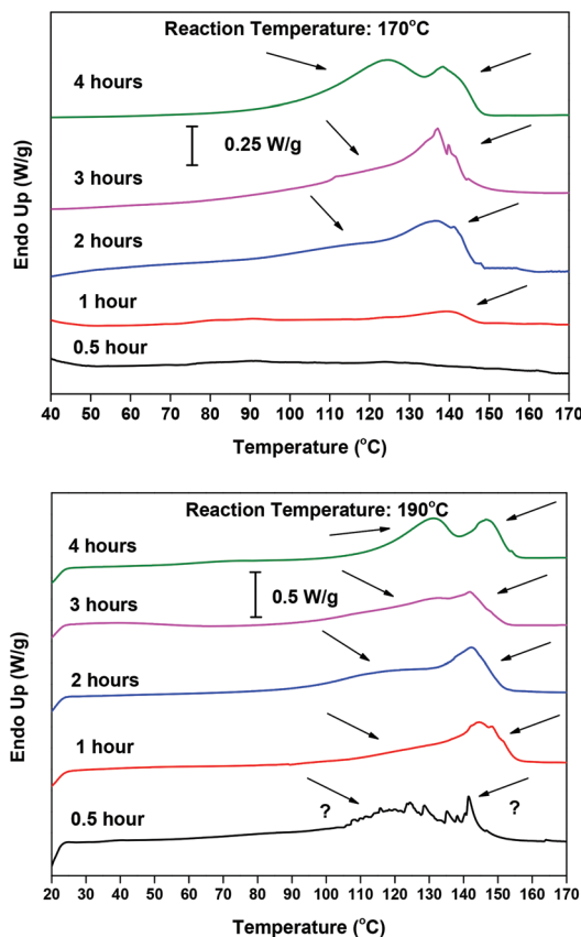
Fig. 4 DSC thermographs of the reaction samples of the esterification step, catalyzed by \text{Sb}_2\text{O}_3 at 170\text{ }^\circ\text{C} (up) and 190\text{ }^\circ\text{C} (down), at different reaction times.
