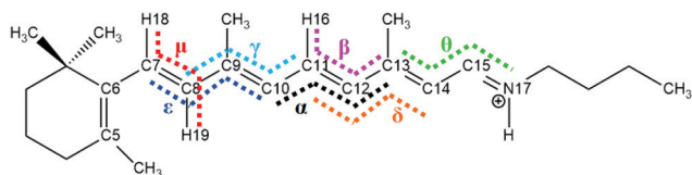
Fig. 1 The numbering of atoms in the backbone of all- trans RPSB. Seven specific dihedral angles (arranged from left to right) are important for the conical intersections, namely \epsilon : C_7C_8C_9C_{10} ; \mu : H_{18}C_7C_8H_{19} ; \gamma : C_8C_9C_{10}C_{11} ; \alpha : C_{10}C_{11}C_{12}C_{13} ; \beta : H_{16}C_{11}C_{12}C_{13} ; \delta : C_{11}C_{12}C_{13}C_{14} ; and \theta : C_{13}C_{14}C_{15}N_{17} .
