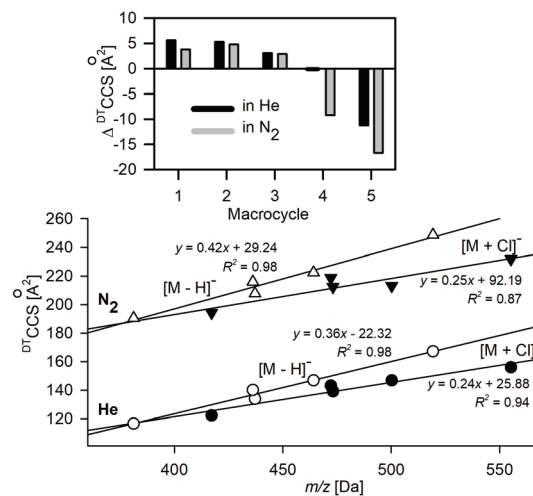
Fig. 1 Relationship between m/z and ^{DT}CCS_{He/N_2} values obtained from direct measurements of deprotonated macrocycles [M – H] − (open symbols) and macrocyclic complexes with Cl − (black symbols). The top part shows the directions of the CCS shifts upon Cl − complexation.
