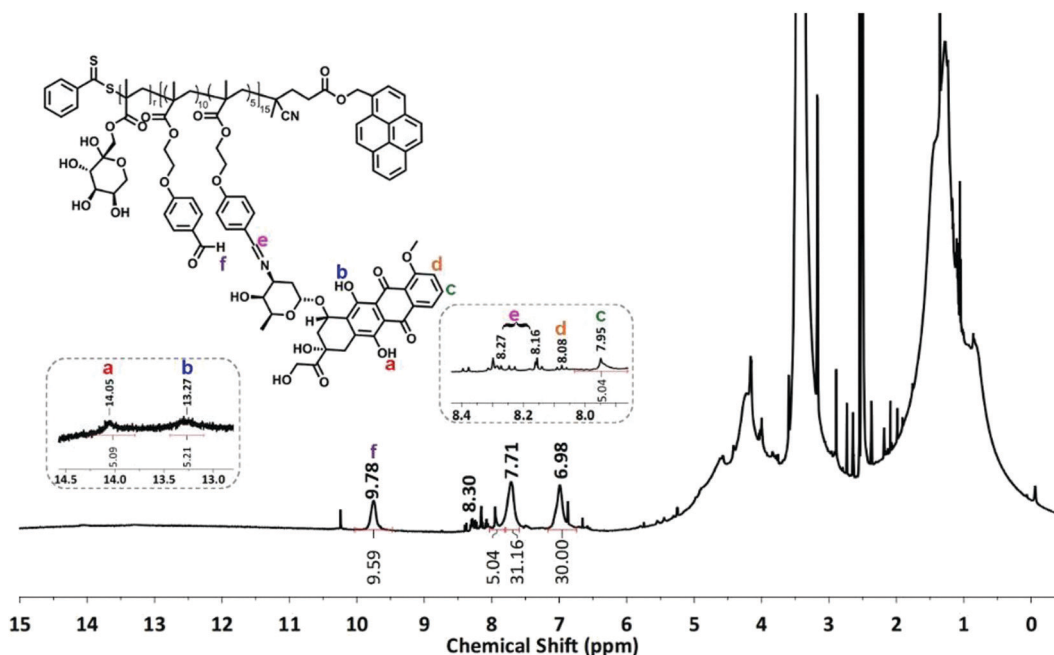
Fig. 1 1 H-NMR spectrum of P(FruMA- b -MAEBAs)-Py/DOX (P7) in CDCl 3 (500 MHz).
