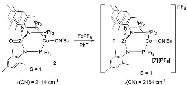
Scheme 3 Chemical oxidation of 2 with \text{FcPF}_6 .
