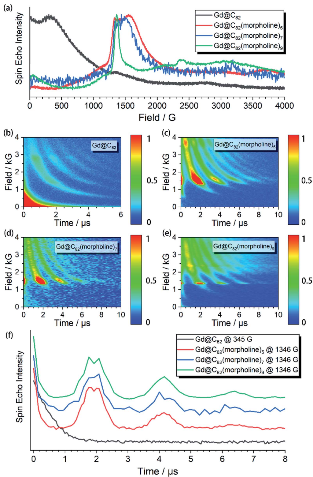
Fig. 2 (a) Echo-detected field swept spectra of Gd@C 82 and the three derivatives Gd- n with normalized echo intensities; (b)–(e) the spin echo decay at different external applied magnetic fields (B 0 ) of each compound; (f) decay of the Hahn-echo intensity as a function of delay time for Gd@C 82 and the three derivatives Gd- n at specific B 0 .
