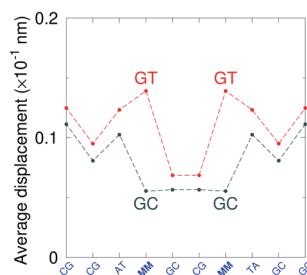
Fig. 10 Average displacements for sequences with GT al mismatches {AgC/TtG} (red curves) and corresponding canonical base pairs (dark grey curves). The calculation was carried out at 180 K, which has no relation to the melting temperatures. Sequences from ref. 97.
