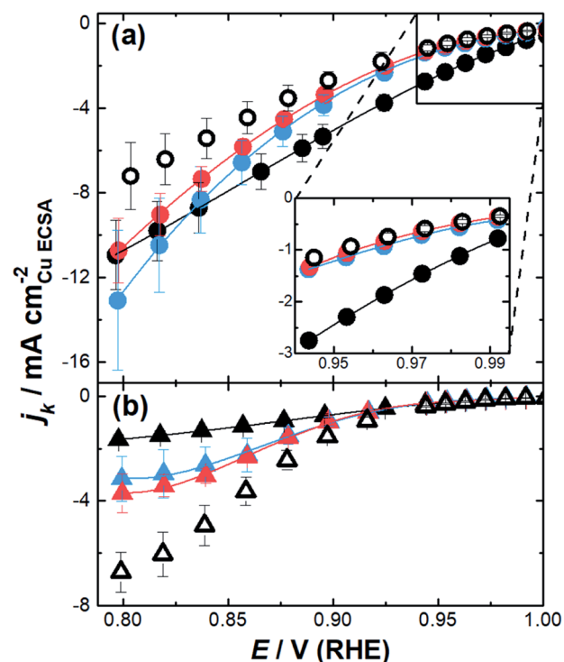
Fig. 4 Kinetic current densities calculated from Koutecký–Levich plots from 0.8–1.0 V (RHE) for (a) NZ small (black), NZ medium (blue), NZ large (red), and mesoporous particles with and without surfactant (white); (b) small channel particles without the surfactant (black), medium channel particles without the surfactant (blue), large channel particles without the surfactant (red), and mesoporous particles without the surfactant (white). The error bars in the inset are smaller than the size of the dots.
