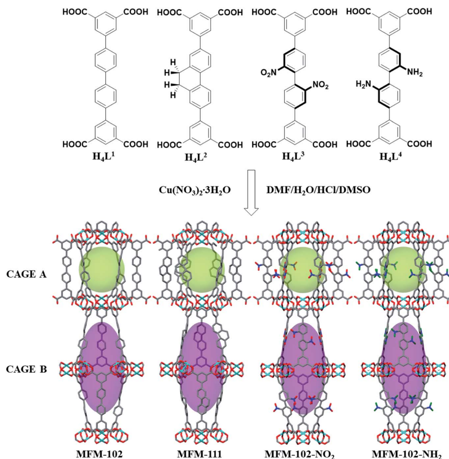
Fig. 1 Views of organic ligands used to construct the MFM-102 series of MOFs and the X-ray crystal structures of MFM-102, MFM-111, MFM-102- NO_2 and MFM-102- NH_2 . The functional groups are highlighted in ball-stick mode. (C, dark grey; O, red; N, blue; Cu, turquoise; all coordinated H_2O and hydrogen atoms are omitted for clarity, except for the hydrogen atoms on the -NH_2 group, green).
