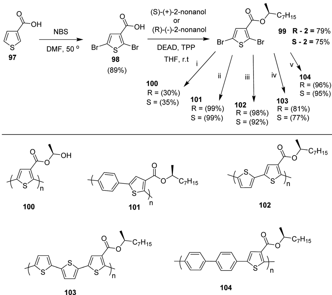
Scheme 32 Synthesis of polythiophene and thiophene-based copolymers with chiral nonyloxy carbonyl substituents. Reagents and conditions: (i) \text{Ni(cod)}_2 , bpy, DMF, 80^\circ\text{C} ; (ii) 95 , \text{Pd(PPh}_3)_4 , \text{NaHCO}_3 , THF, \text{H}_2\text{O} , reflux; (iii) 94 , \text{Pd}_2(\text{dba})_3 , TFP, THF, 50^\circ\text{C} ; (iv) 93 , \text{Pd}_2(\text{dba})_3 , TFP, THF, 50^\circ\text{C} ; (v) 96 , \text{Pd(PPh}_3)_4 , \text{NaHCO}_3 , THF, \text{H}_2\text{O} , reflux.
