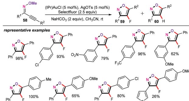
Scheme 27 Gold-catalyzed cascade cyclization/fluorination reaction.
