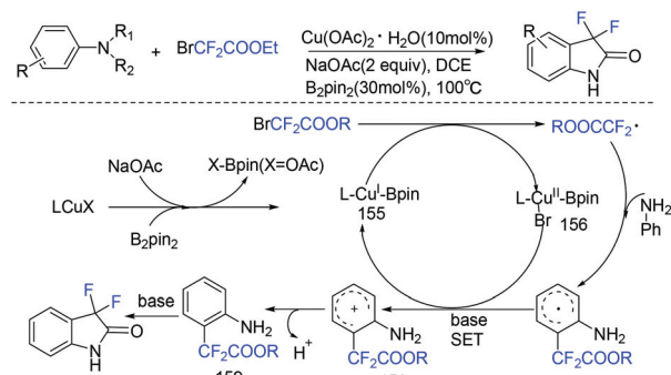
Scheme 99 The copper/B 2 pin 2 -catalyzed C–H difluoroacetylation–cycloamidation of anilines.
