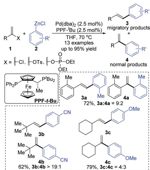
Scheme 2 Skrydstrup's Negishi couplings involving a 1,2-palladium migration process.
