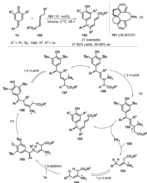
Scheme 40 Enantioselective dienylation of p -QMs.
