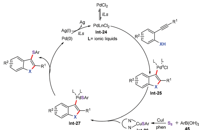
Scheme 19 Plausible mechanism for palladium-catalyzed cascade annulation/aryltiolation reaction.
