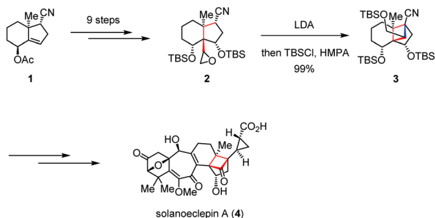
Scheme 1 Intramolecular nucleophilic cyclization in the total synthesis of solanoecclepin A.
