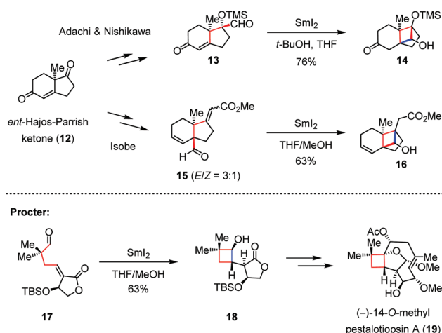
Scheme 3 Ketyl-olefin radical cyclizations in the syntheses of solanoecclepin A and (–)-14- O -methyl pestalotiopsin A.
