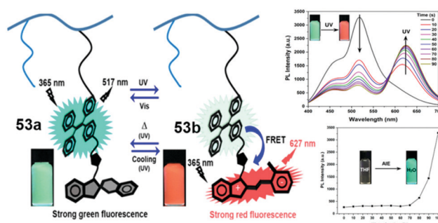
Fig. 24 Schematic illustration of the energy transfer from the TPE to MC unit via the FRET process after UV exposure and the AIE property of 53a in THF/H_2O solutions. Reproduced with permission. 65 Copyright 2020, American Chemical Society.
