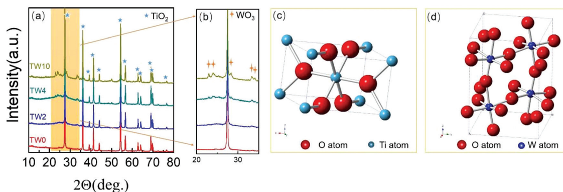
Fig. 2 (a) XRD patterns and (b) magnified XRD patterns in the region of 20–35 degrees of TW0, TW2, TW4 and TW10. (c) TiO 2 and (d) WO 3 unit cell images.
