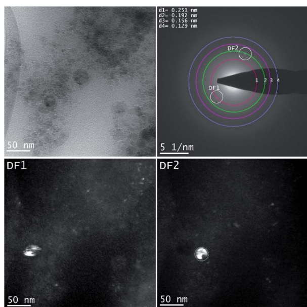
Fig. 7 The femtosecond laser-synthesized Si nanoparticles in n -hexane. ( N = 1000 , F = 10.46 \text{ J cm}^{-2} ). The TEM bright-field image, SAED pattern (upper right) and dark-field images related to different diffracted electron beams along the 1 st and 2 nd ring. The EDX spectrum from several small Si NPs and one Si NP.
